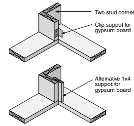
Two-stud Corner
